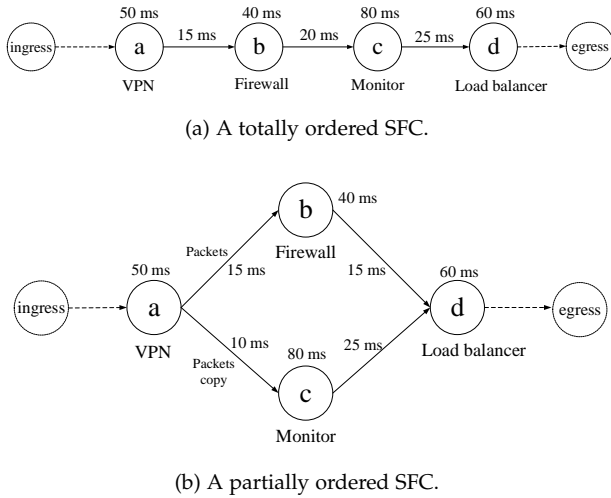
Fig. 3: Totally ordered SFC v.s. partially ordered SFC, derived from [28].
