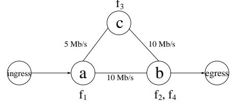
Fig. 1: An example of describing the VPTR problem.
