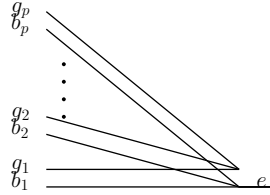
Fig. 1. The bad flows are denoted by b with an index, while the good ones are denoted by g with an index. The paths of flow b_i and g_i coincide, besides edge e , belonging only to the bad flows.
